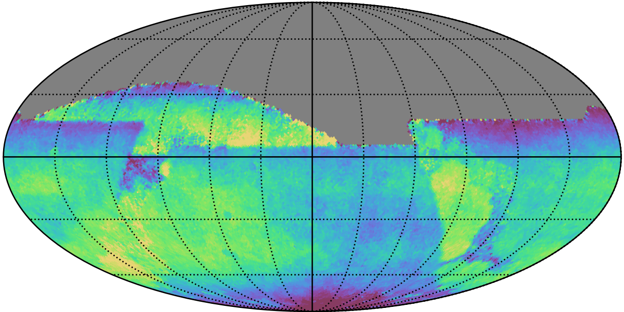
ddf_acor_sf10_lsf20_lsr10_v3.4_10yrs All sky all bands: Median fiveSigmaDepth
