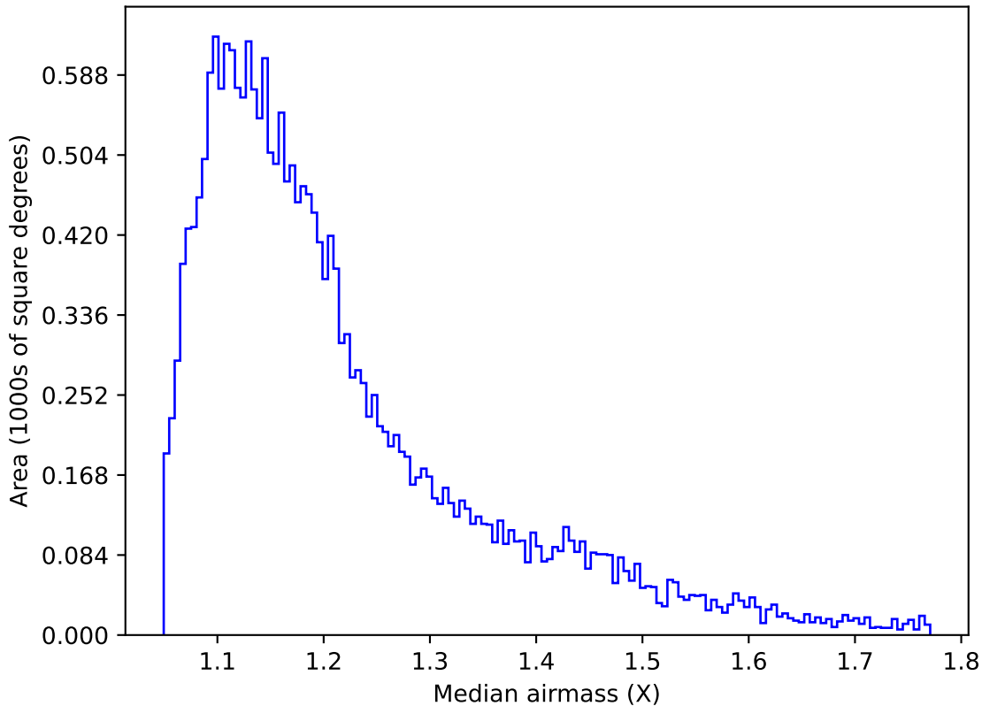
ddf_acor_sf10_lsf20_lsr10_v3.4_10yrs Yr 1 u band: Median airmass
