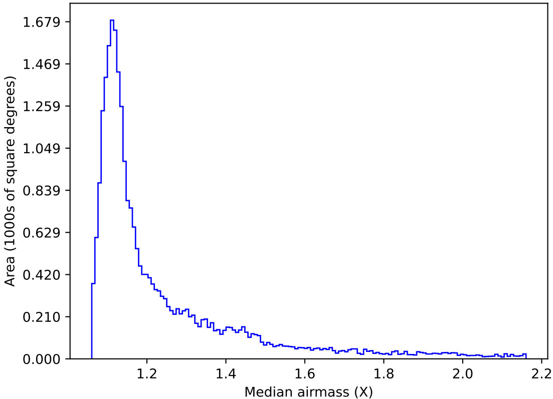
ddf_acor_sf10_lsf20_lsr10_v3.4_10yrs Yr 1 i band: Median airmass
