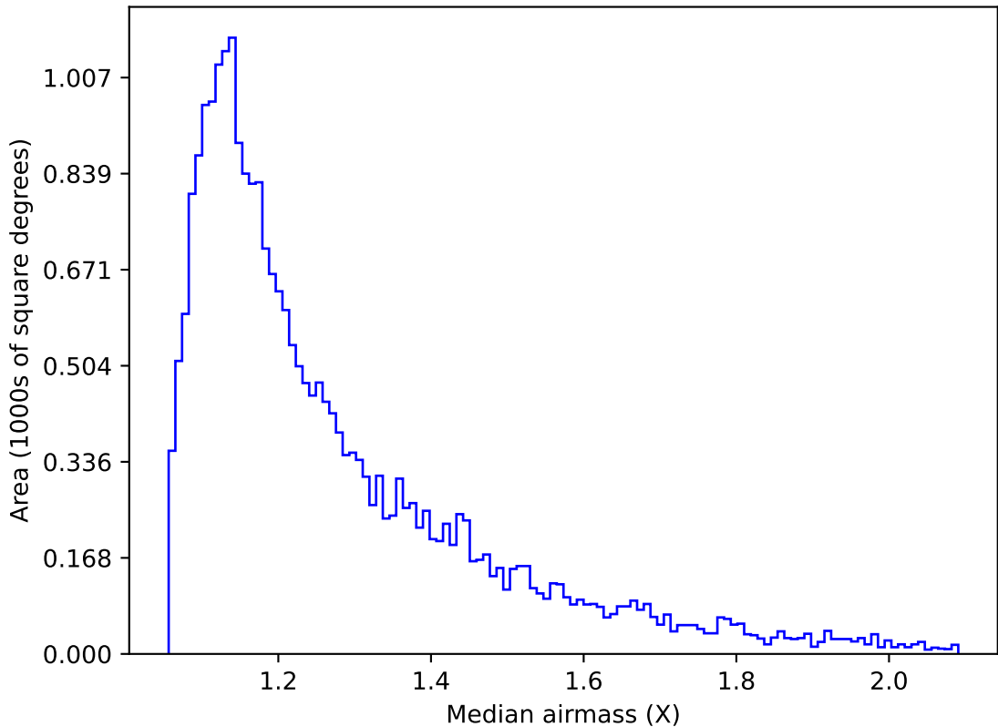
ddf_acor_sf10_lsf20_lsr10_v3.4_10yrs Yr 1 g band: Median airmass
