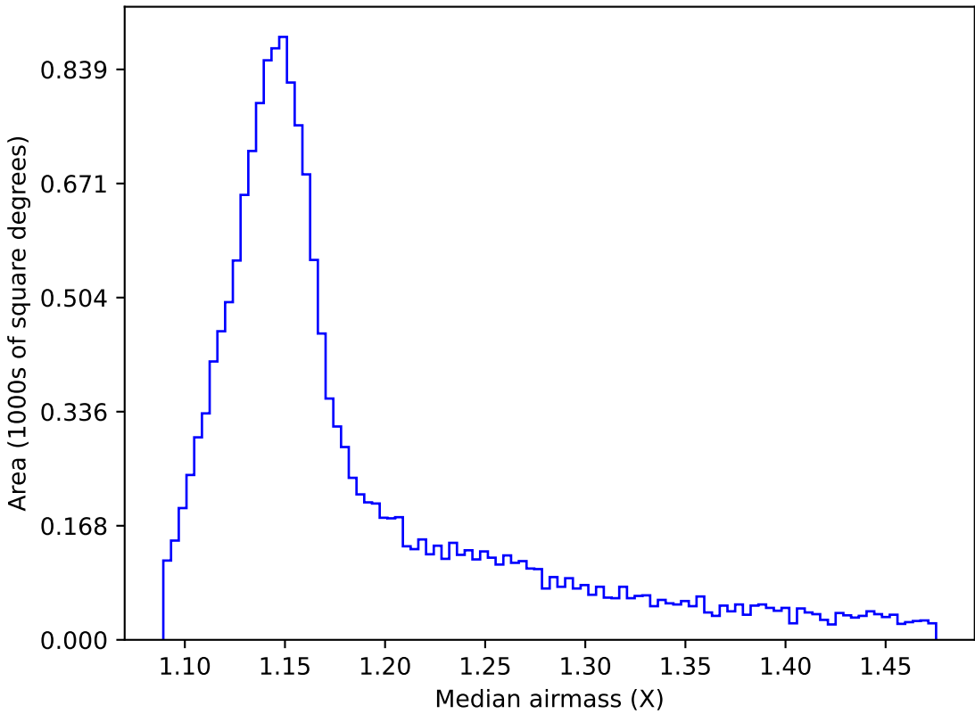
ddf_acor_sf10_ls20_lsr10_v3.4_10yrs WFD y band: Median airmass
