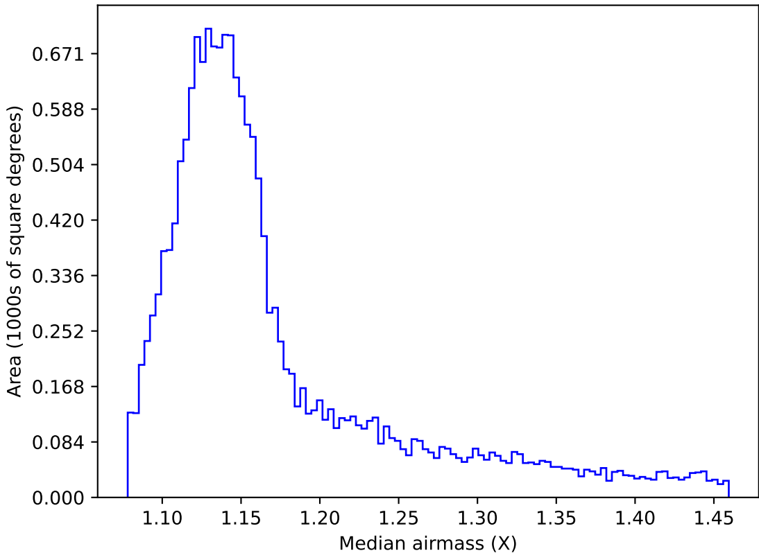
ddf_acor_sf10_lsf20_lsr10_v3.4_10yrs WFD i band: Median airmass
