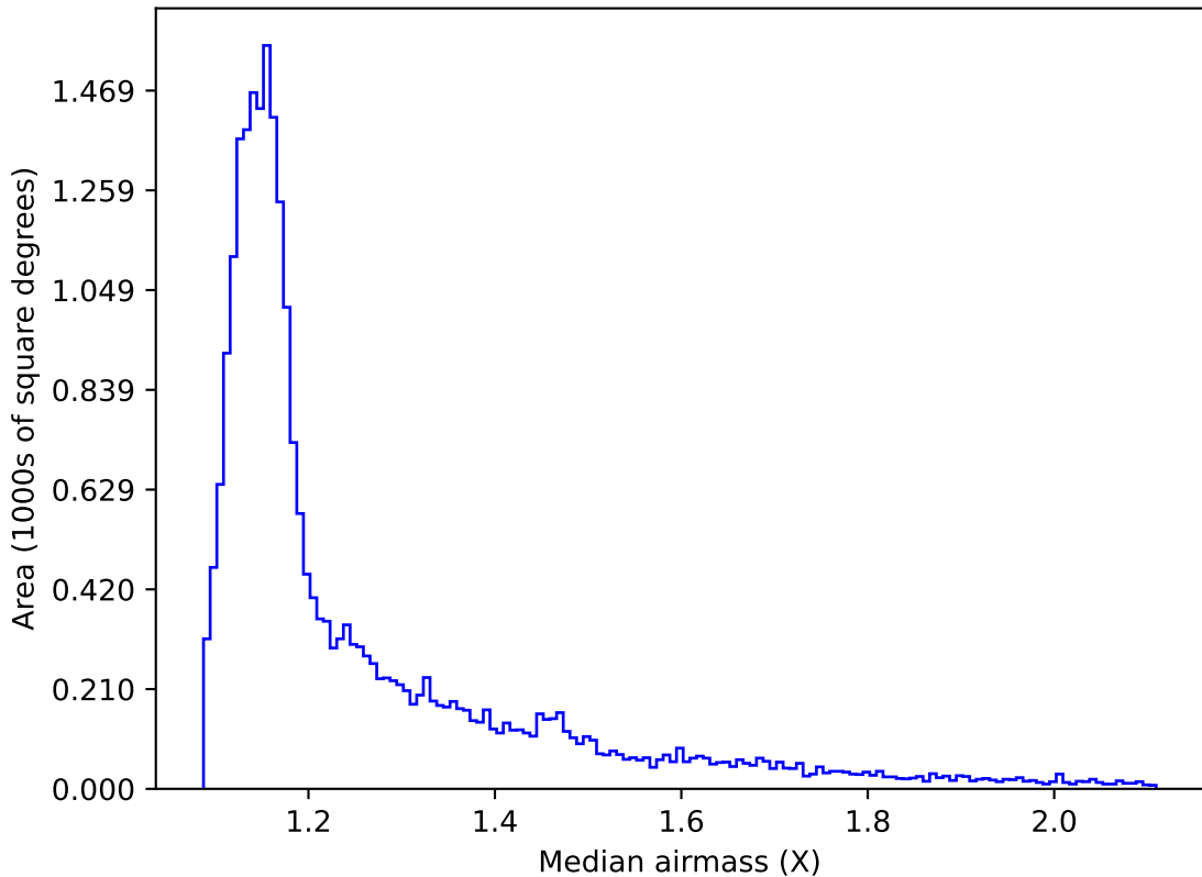
ddf_acor_sf10_lsf20_lsr10_v3.4_10yrs All sky z band: Median airmass
