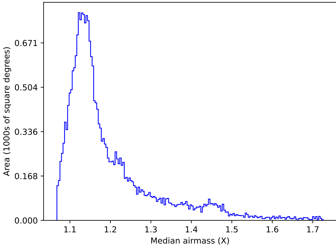
ddf_acor_sf10_lsf20_lsr10_v3.4_10yrs All sky u band: Median airmass
