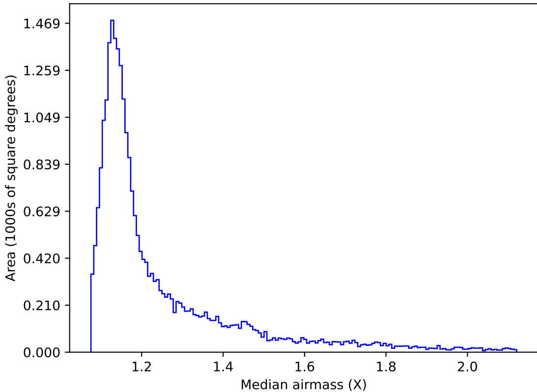
ddf_acor_sf10_lsf20_lsr10_v3.4_10yrs All sky g band: Median airmass
