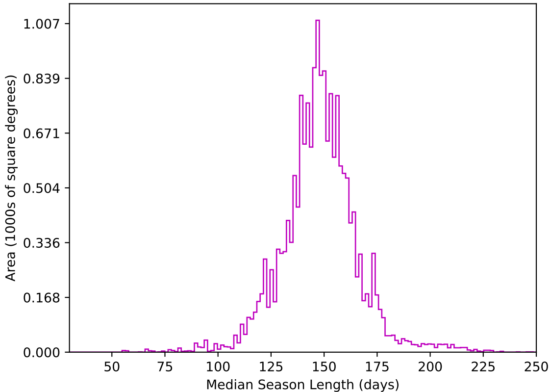
ddf_acor_sf10_lsf20_lsr10_v3.4_10yrs WFD z band: Median Season Length
