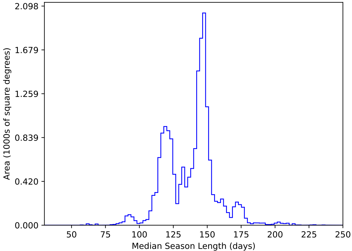
ddf_acor_sf10_lsf20_lsr10_v3.4_10yrs WFD y band: Median Season Length
