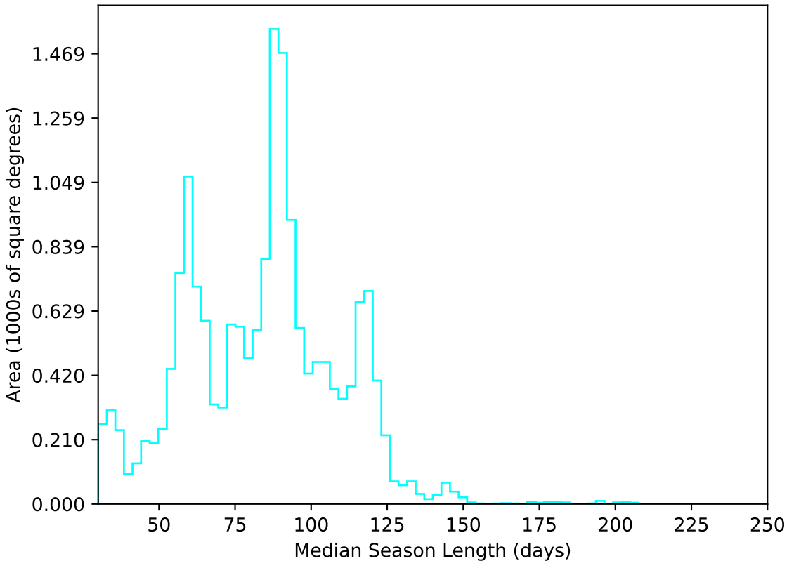
ddf_acor_sf10_lsf20_lsr10_v3.4_10yrs WFD u band: Median Season Length
