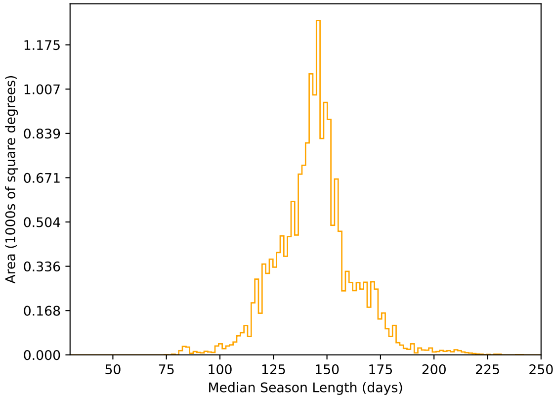
ddf_acor_sf10_lsf20_lsr10_v3.4_10yrs WFD r band: Median Season Length
