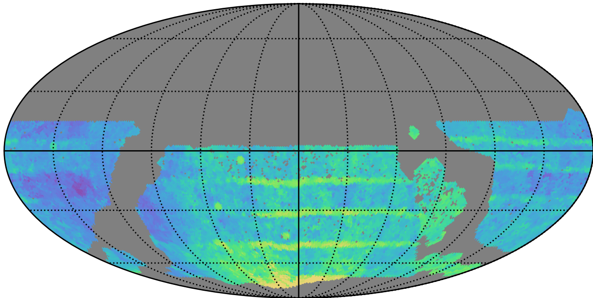
ddf_acor_sf10_lsf20_lsr10_v3.4_10yrs WFD all bands: Median Season Length
