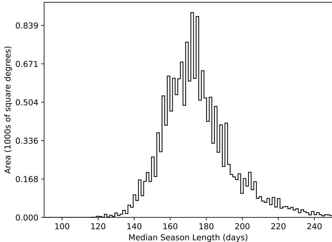
ddf_acor_sf10_lsf20_lsr10_v3.4_10yrs WFD all bands: Median Season Length
