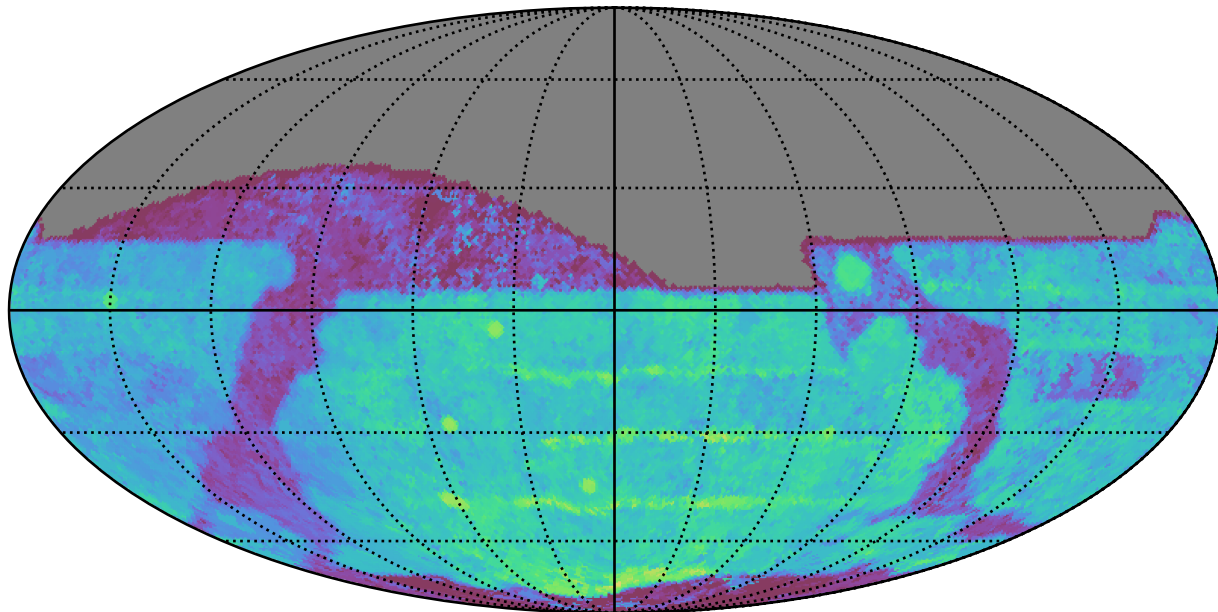
ddf_acor_sf10_lsf20_lsr10_v3.4_10yrs All sky z band: Median Season Length
