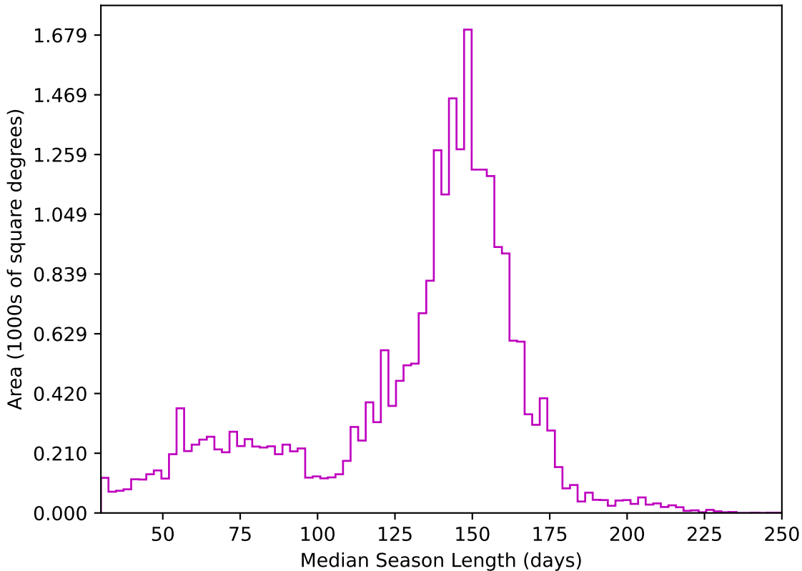
ddf_acor_sf10_lsf20_lsr10_v3.4_10yrs All sky z band: Median Season Length
