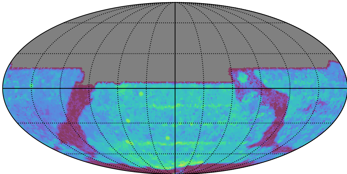
ddf_acor_sf10_lsf20_lsr10_v3.4_10yrs All sky y band: Median Season Length
