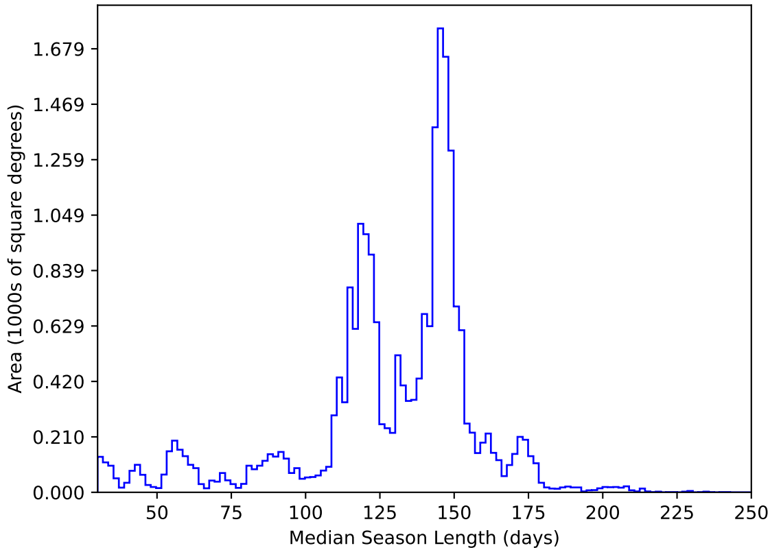
ddf_acor_sf10_lsf20_lsr10_v3.4_10yrs All sky y band: Median Season Length
