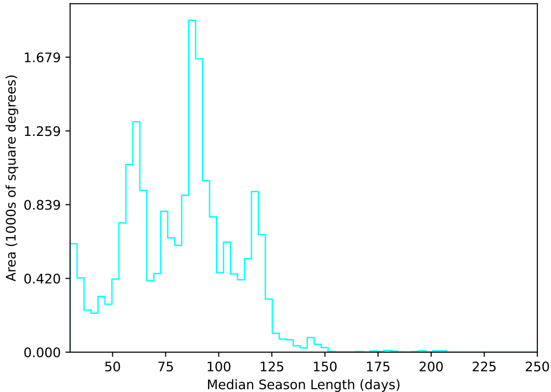
ddf_acor_sf10_lsf20_lsr10_v3.4_10yrs All sky u band: Median Season Length
