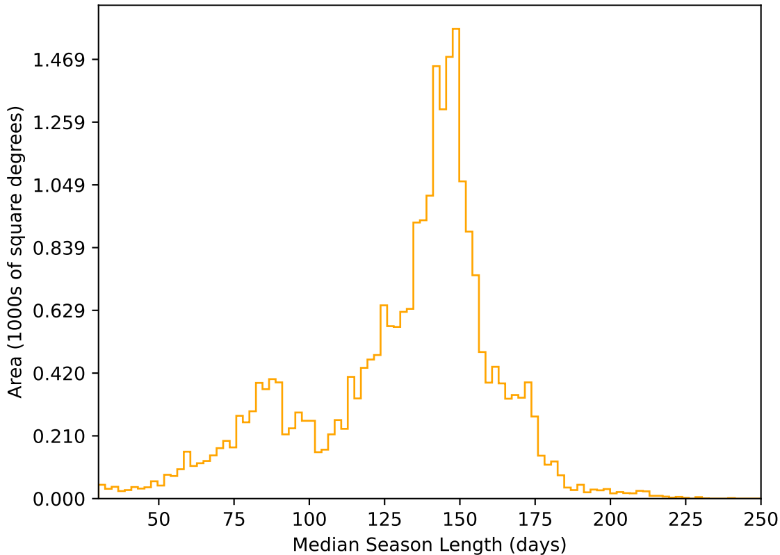
ddf_acor_sf10_lsf20_lsr10_v3.4_10yrs All sky r band: Median Season Length
