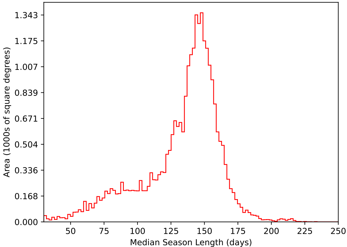
ddf_acor_sf10_lsf20_lsr10_v3.4_10yrs All sky i band: Median Season Length
