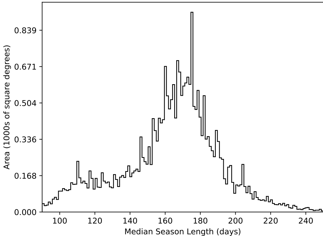
ddf_acor_sf10_lsf20_lsr10_v3.4_10yrs All sky all bands: Median Season Length
