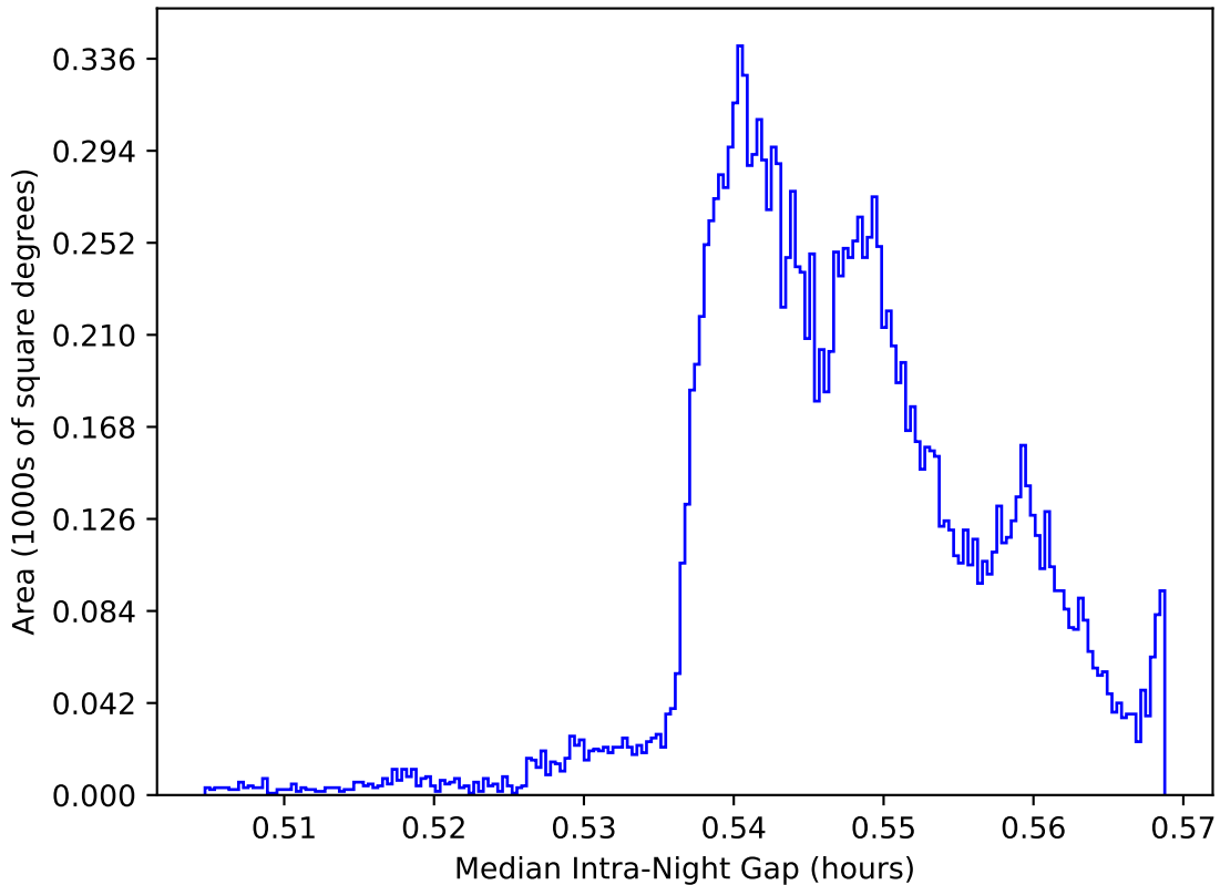
ddf_acor_sf10_lsf20_lsr10_v3.4_10yrs WFD: Median Intra-Night Gap
