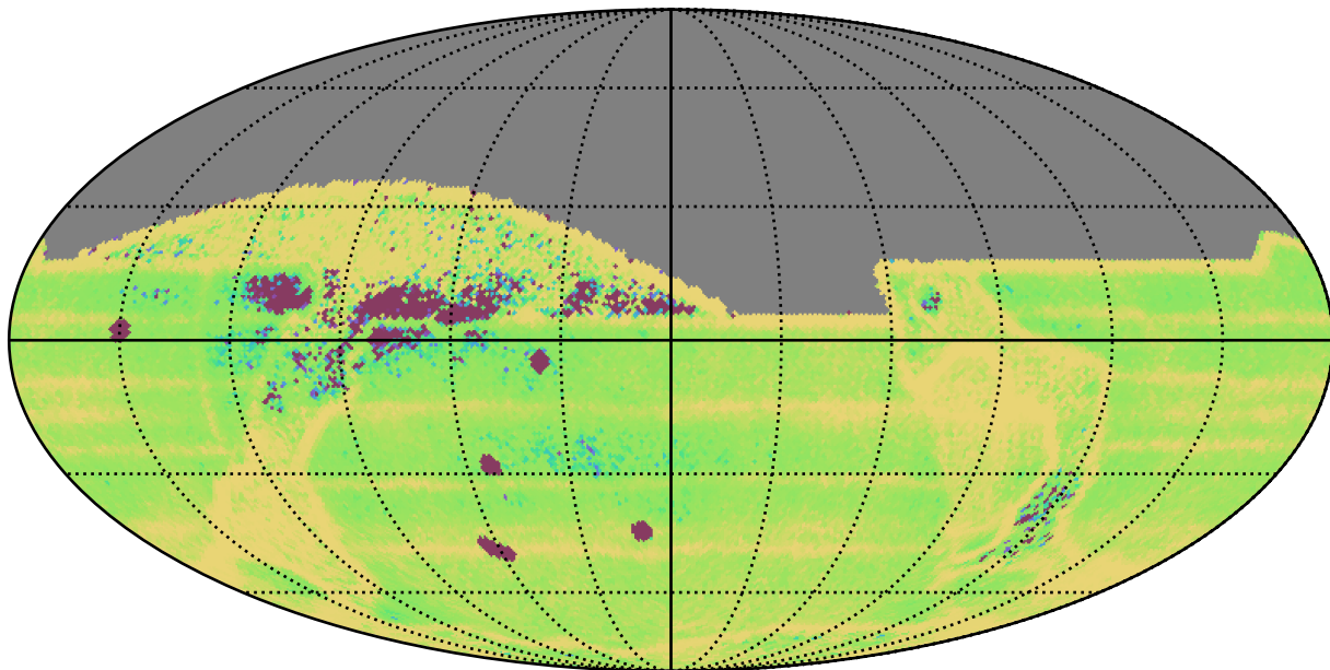
ddf_acor_sf10_lsf20_lsr10_v3.4_10yrs All sky: Median Intra-Night Gap
