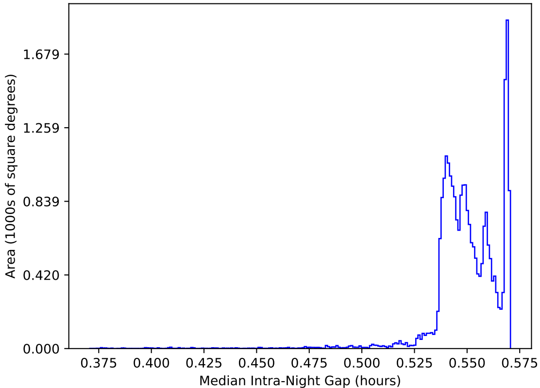
ddf_acor_sf10_lsf20_lsr10_v3.4_10yrs All sky: Median Intra-Night Gap
