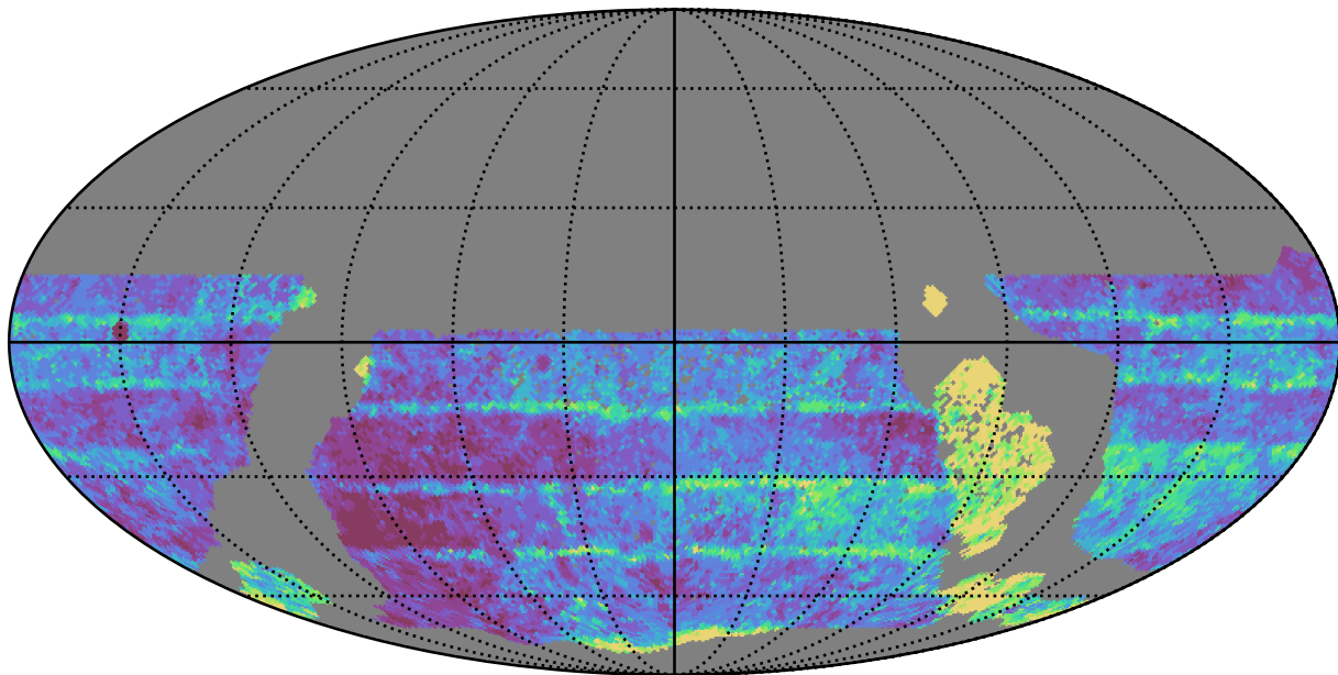
ddf_acor_sf10_lsf20_lsr10_v3.4_10yrs WFD z band: Median Inter-Night Gap
