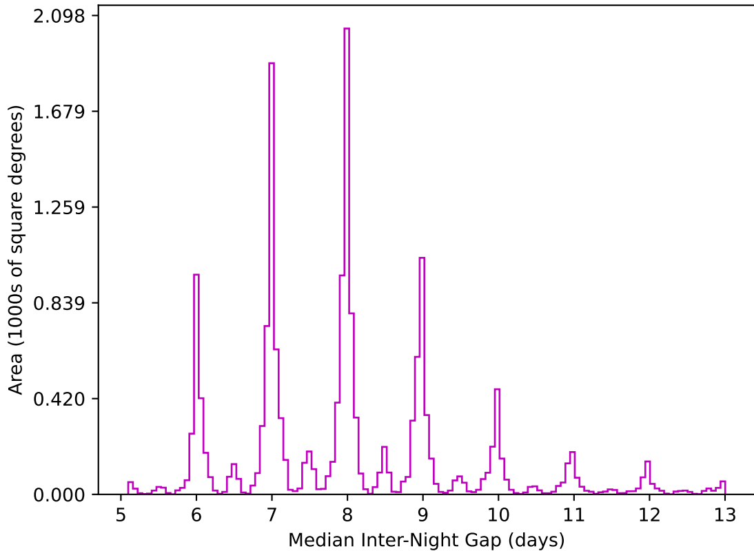
ddf_acor_sf10_lsf20_lsr10_v3.4_10yrs WFD z band: Median Inter-Night Gap
