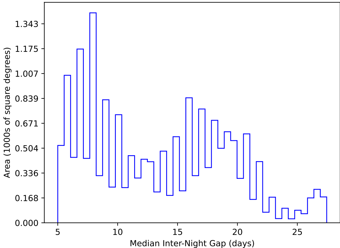
ddf_acor_sf10_lsf20_lsr10_v3.4_10yrs WFD y band: Median Inter-Night Gap
