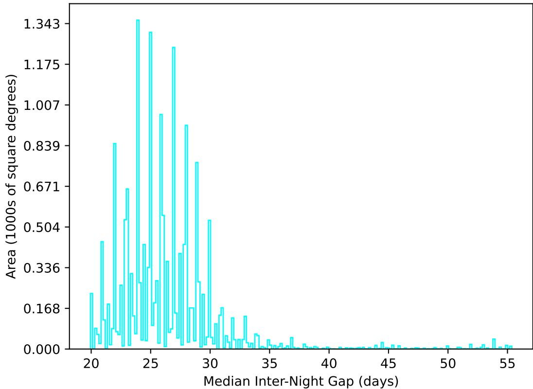
ddf_acor_sf10_lsf20_lsr10_v3.4_10yrs WFD u band: Median Inter-Night Gap
