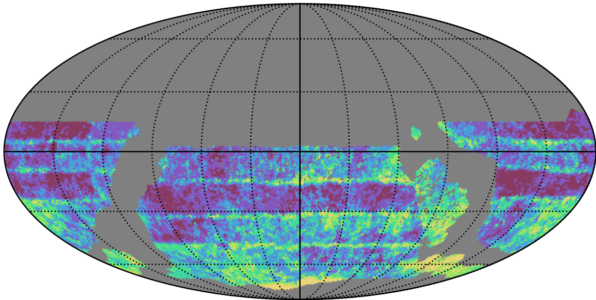
ddf_acor_sf10_lsf20_lsr10_v3.4_10yrs WFD r band: Median Inter-Night Gap
