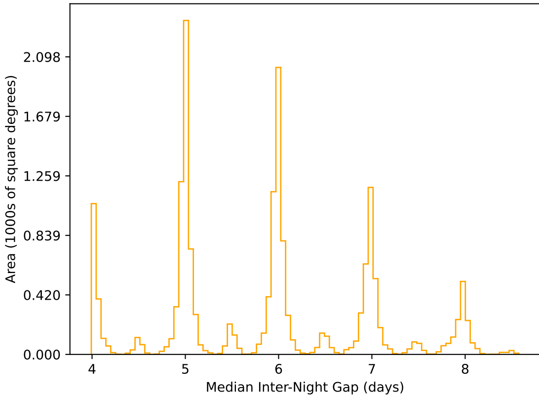
ddf_acor_sf10_lsf20_lsr10_v3.4_10yrs WFD r band: Median Inter-Night Gap
