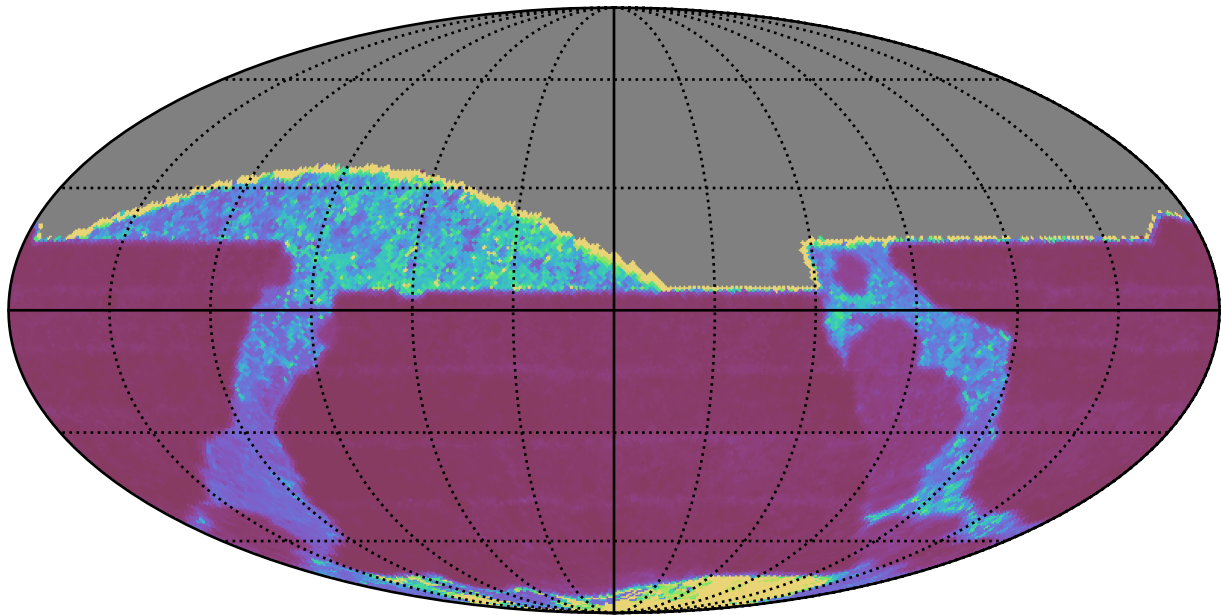
ddf_acor_sf10_lsf20_lsr10_v3.4_10yrs All sky z band: Median Inter-Night Gap
