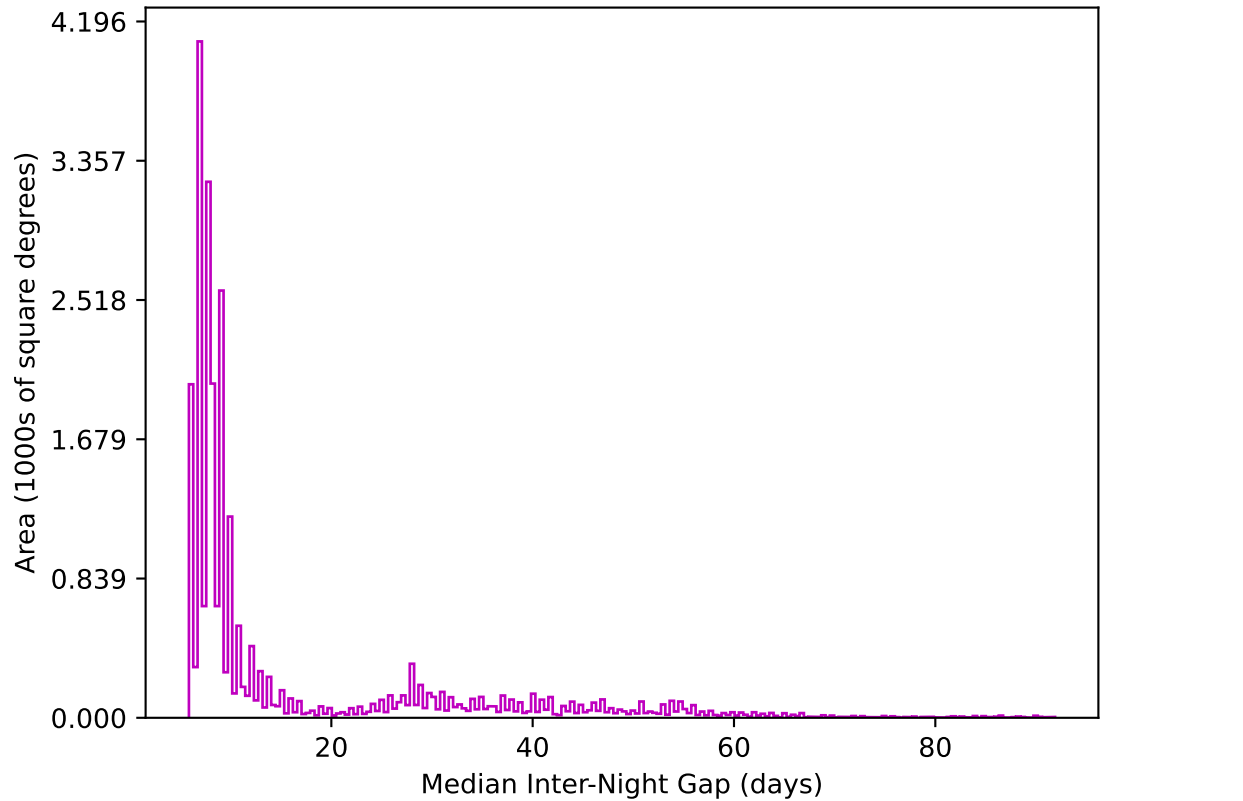
ddf_acor_sf10_lsf20_lsr10_v3.4_10yrs All sky z band: Median Inter-Night Gap
