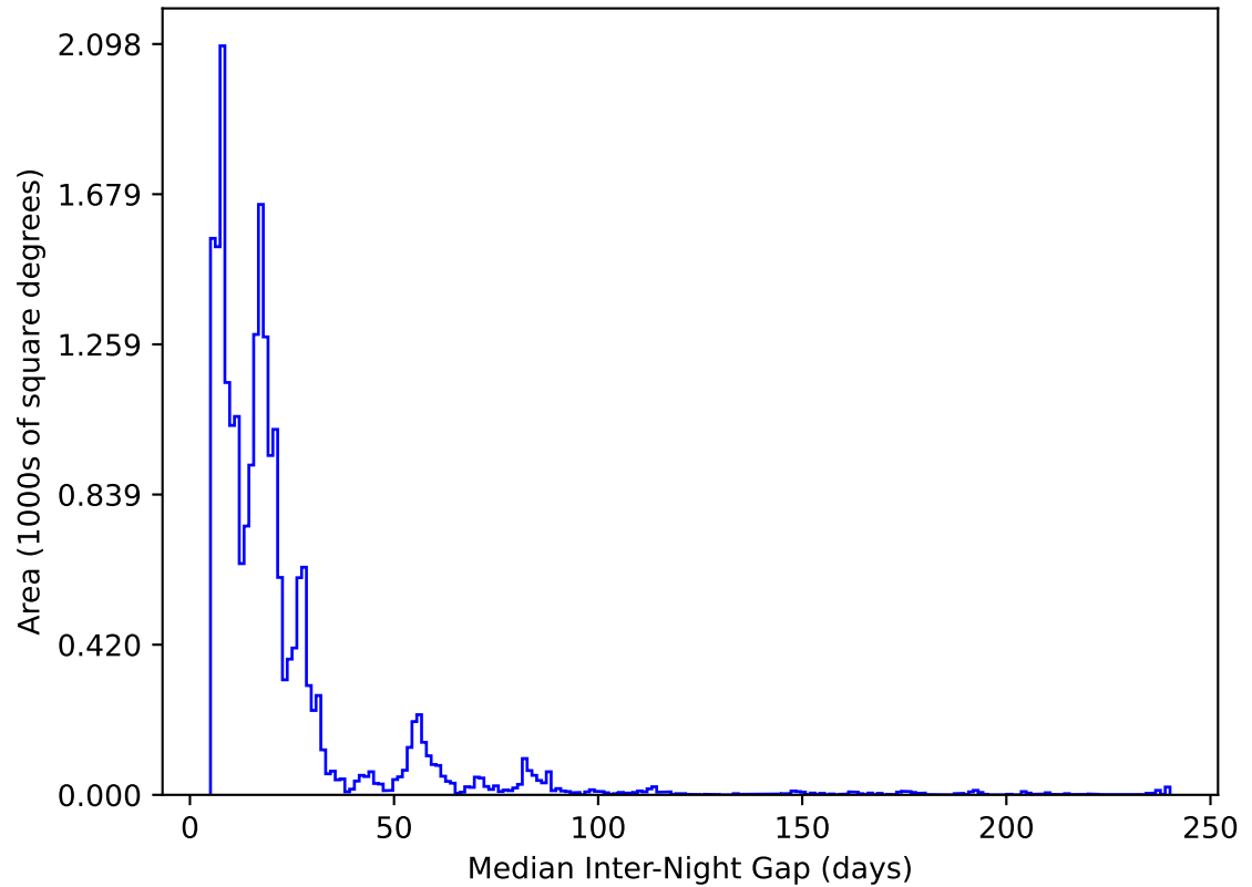
ddf_acor_sf10_lsf20_lsr10_v3.4_10yrs All sky y band: Median Inter-Night Gap
