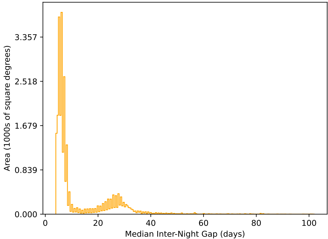
ddf_acor_sf10_lsf20_lsr10_v3.4_10yrs All sky r band: Median Inter-Night Gap
