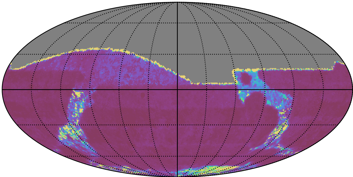
ddf_acor_sf10_lsf20_lsr10_v3.4_10yrs All sky g band: Median Inter-Night Gap
