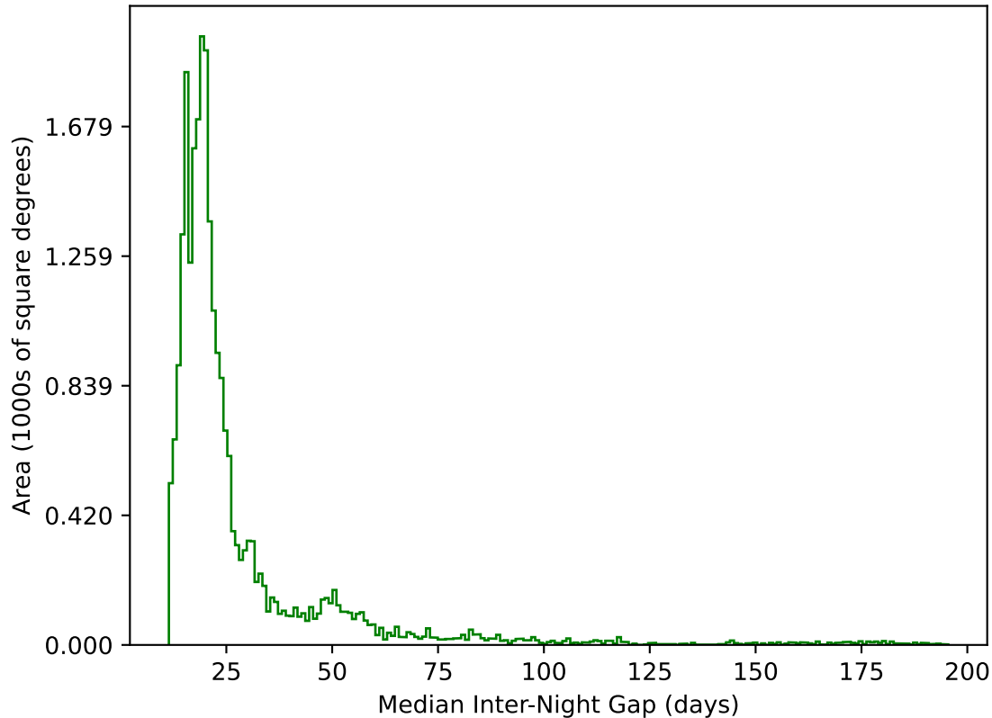
ddf_acor_sf10_lsf20_lsr10_v3.4_10yrs All sky g band: Median Inter-Night Gap
