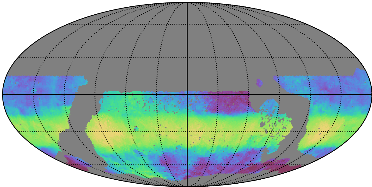
ddf_acor_sf10_lsf20_lsr10_v3.4_10yrs WFD z band: Median HA
