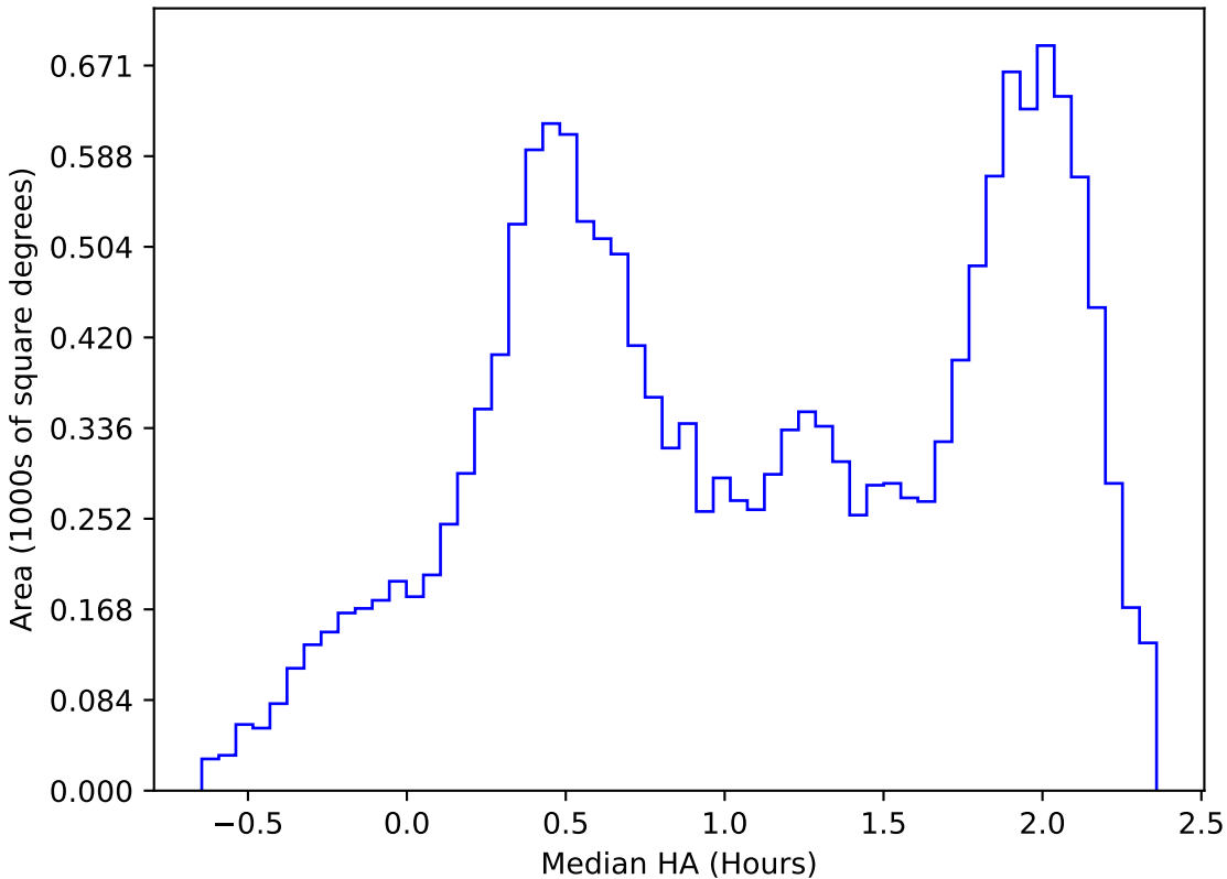
ddf_acor_sf10_lsf20_lsr10_v3.4_10yrs WFD z band: Median HA
