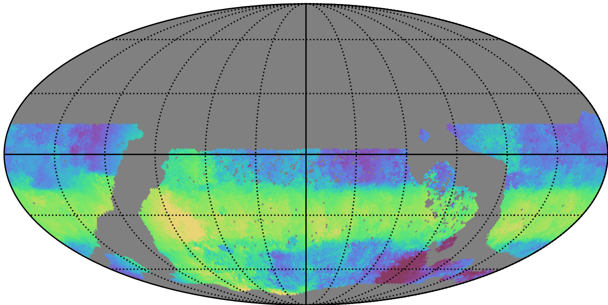
ddf_acor_sf10_lsf20_lsr10_v3.4_10yrs WFD u band: Median HA
