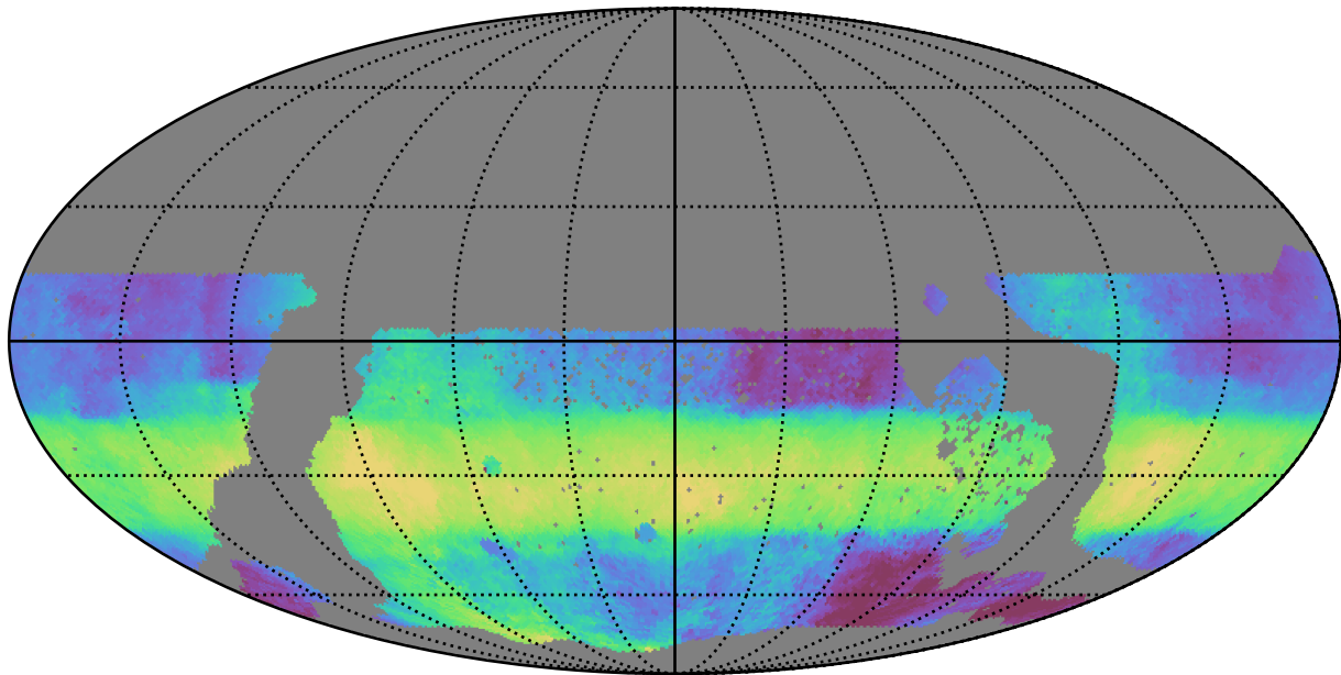
ddf_acor_sf10_lsf20_lsr10_v3.4_10yrs WFD r band: Median HA
