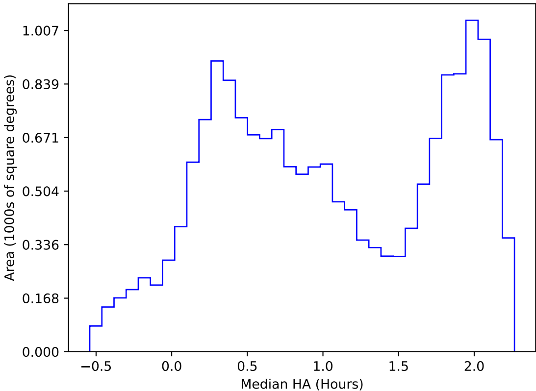
ddf_acor_sf10_lsf20_lsr10_v3.4_10yrs WFD i band: Median HA
