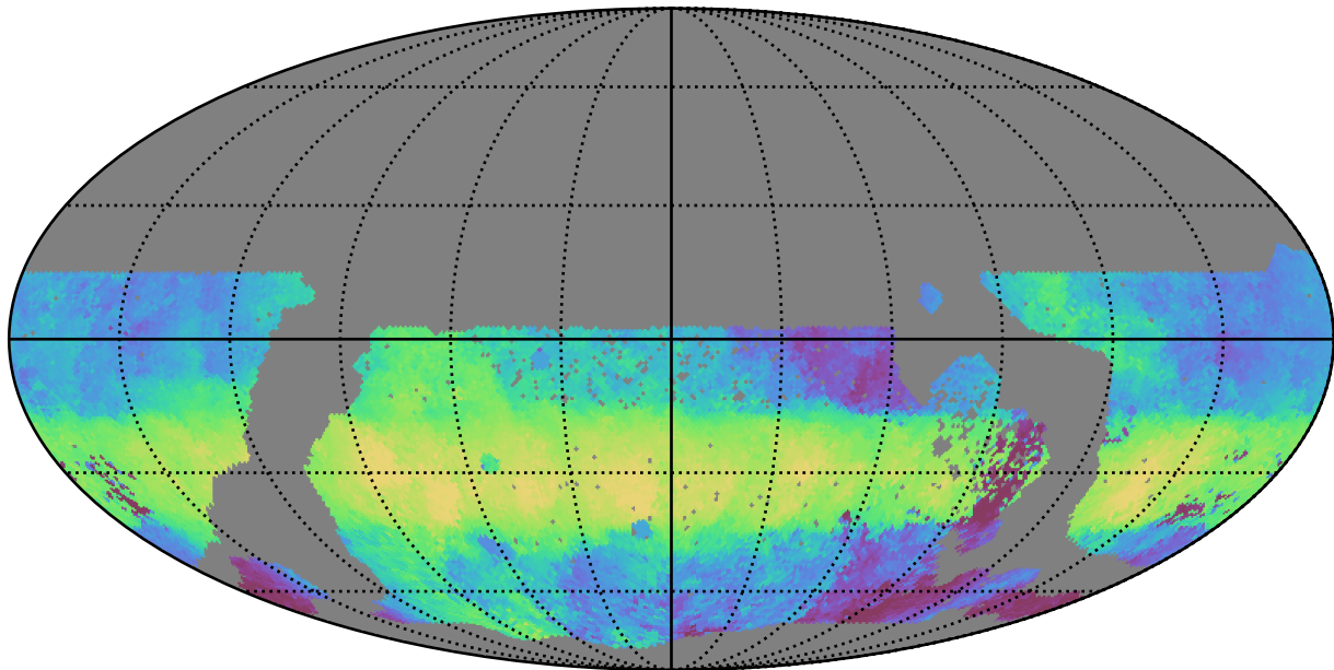
ddf_acor_sf10_lsf20_lsr10_v3.4_10yrs WFD g band: Median HA
