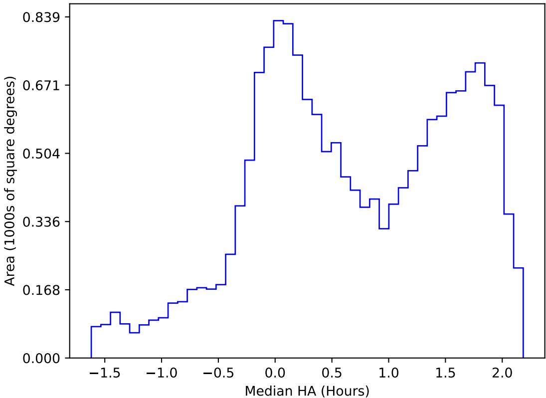
ddf_acor_sf10_lsf20_lsr10_v3.4_10yrs WFD g band: Median HA
