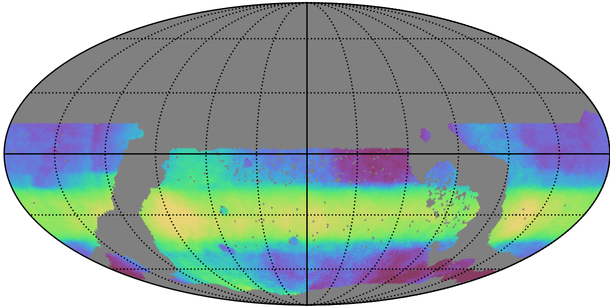
ddf_acor_sf10_lsf20_lsr10_v3.4_10yrs WFD all bands: Median HA
