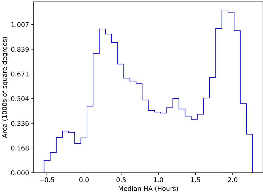
ddf_acor_sf10_lsf20_lsr10_v3.4_10yrs WFD all bands: Median HA
