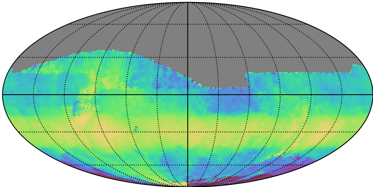
ddf_acor_sf10_lsf20_lsr10_v3.4_10yrs All sky z band: Median HA
