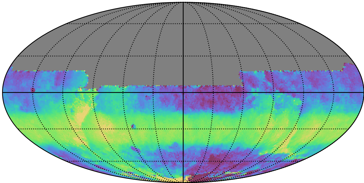
ddf_acor_sf10_lsf20_lsr10_v3.4_10yrs All sky y band: Median HA
