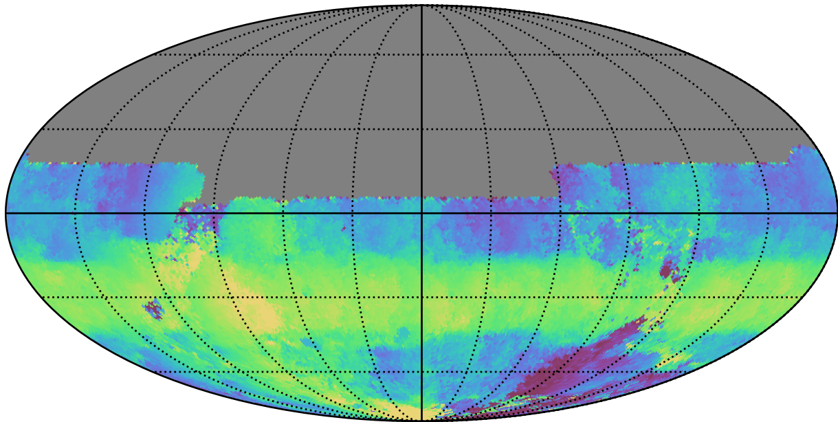
ddf_acor_sf10_lsf20_lsr10_v3.4_10yrs All sky u band: Median HA
